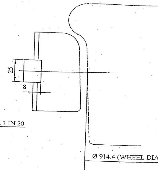
SECTION C-C
